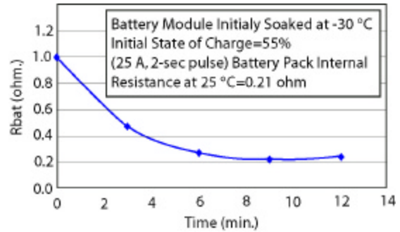
Figure 8. Internal resistance of NiMH battery pack as a function of time after applying AC heat (based on 25A, 2-s pulses)
