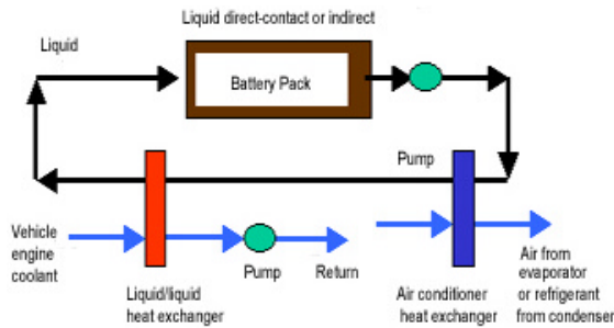
Figure 2. Schematic of liquid heating and cooling
