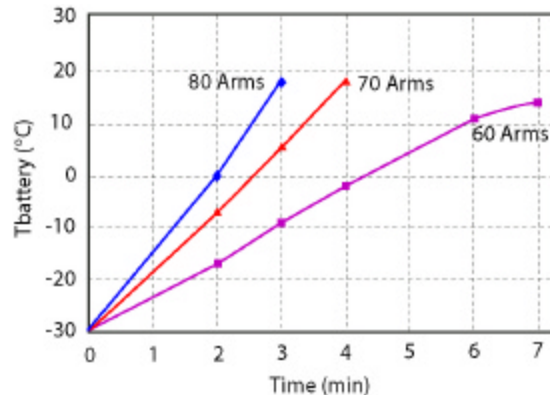
Figure 9. NiMH battery pack temperature as a function of amplitude of AC current (initial battery SOC = 55%) derived from 2-second pulse tests
