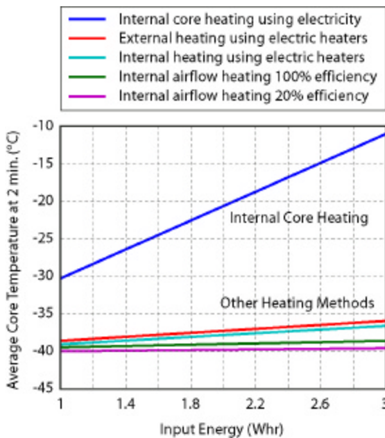
Figure 5. Comparison of various methods to heat a battery with small aspect ratios (width/length)
